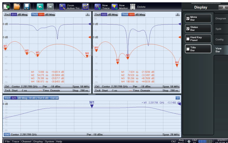
Filter adjustment using time-domain analysis.
